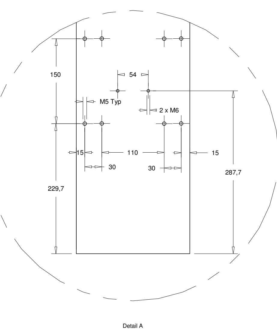
Detail A
